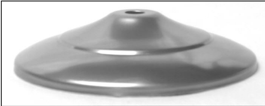
729 4 7/8" ID 1 1/16" high
