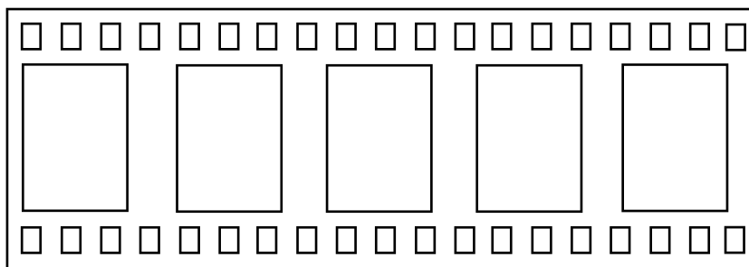
P-1562 (1 9/16") Large holes - 1" x 0.625" Small holes - 0.124" x 0.09"
