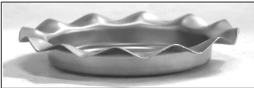
680 4 9/16" OD 3 7/16" ID 13/16" high
