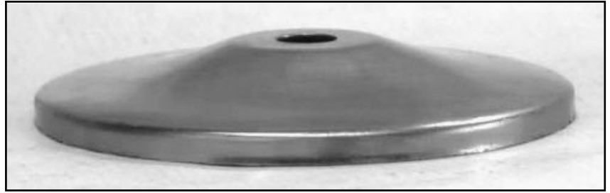
564 3 9/16" ID 7/8" high Fits A50 series bodies/cups
